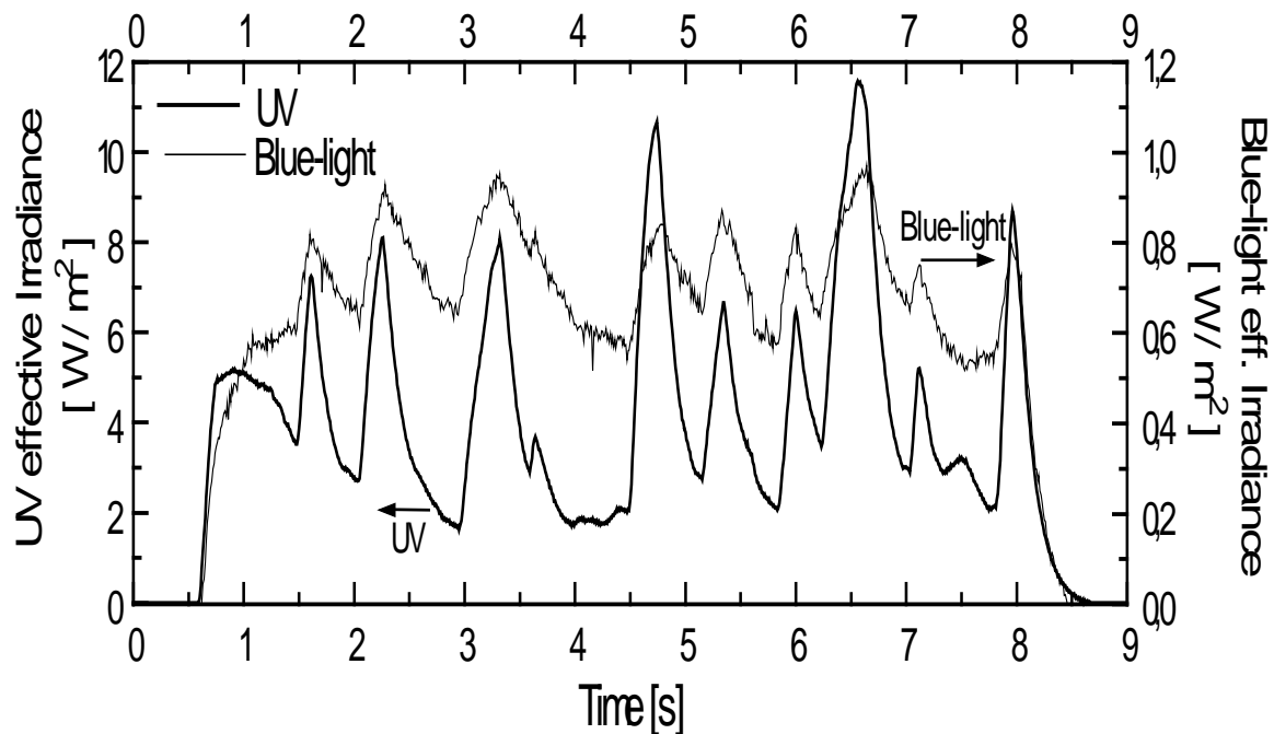
Figure 2. The irradiance maxima result from plasma shielding, where emissions particularly in the UV are greatly increased; the irradiance minima are equivalent to the values as obtained with optimised processing parameters.
