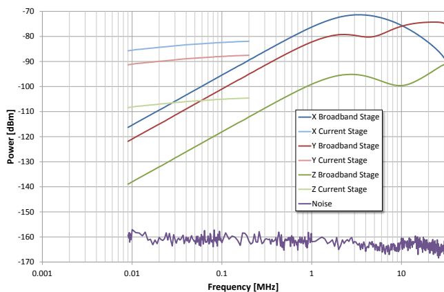
Figure 2: Signal levels for 10 m Normalized Site Insertion Loss (NSIL) measurement using 10 Hz resolution bandwidth
