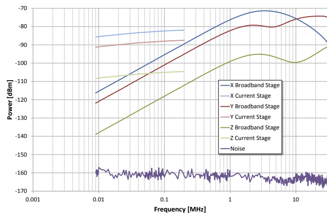
Figure 2: Signal levels for 10 m Normalized Site Attenuation measurement using 10 Hz resolution bandwidth
